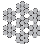
6x7+IWS
