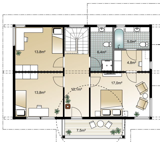
FIRST FLOOR 1:150
