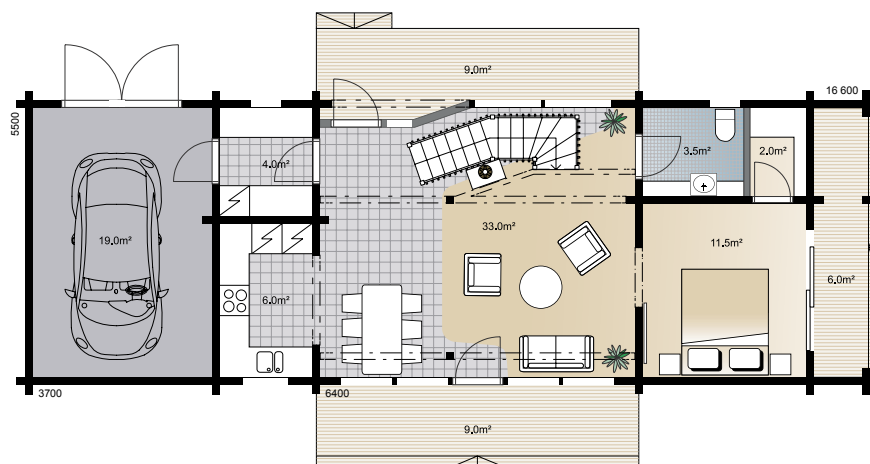
GROUND FLOOR 1:150
