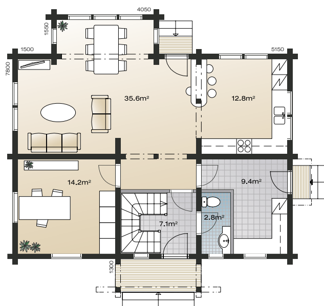
GROUND FLOOR 1:150
