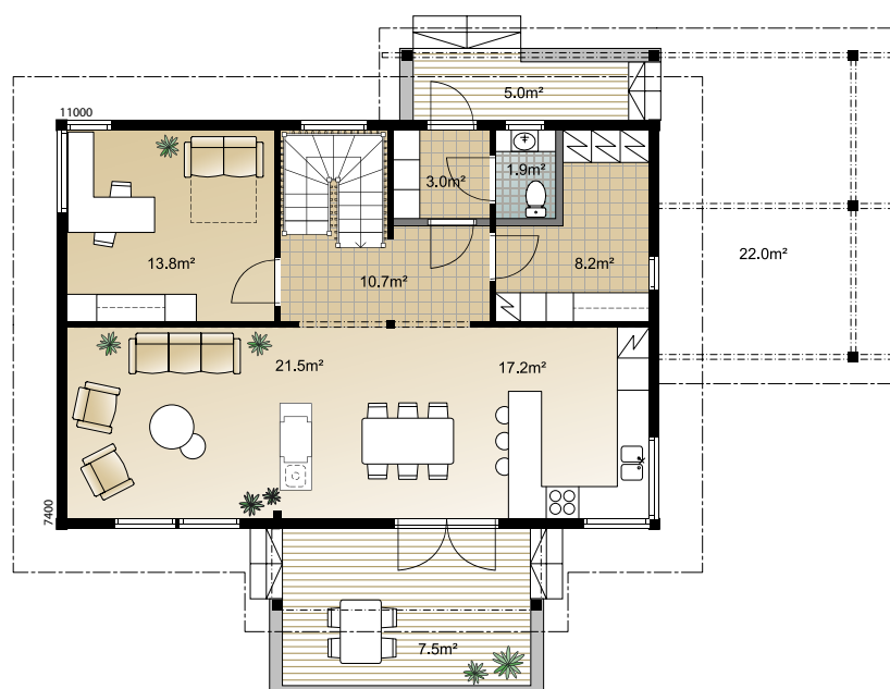
GROUND FLOOR 1:150
