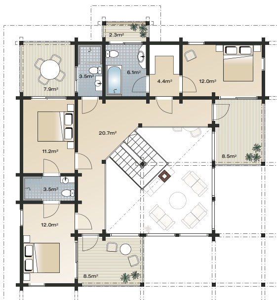
FIRST FLOOR 1:200
