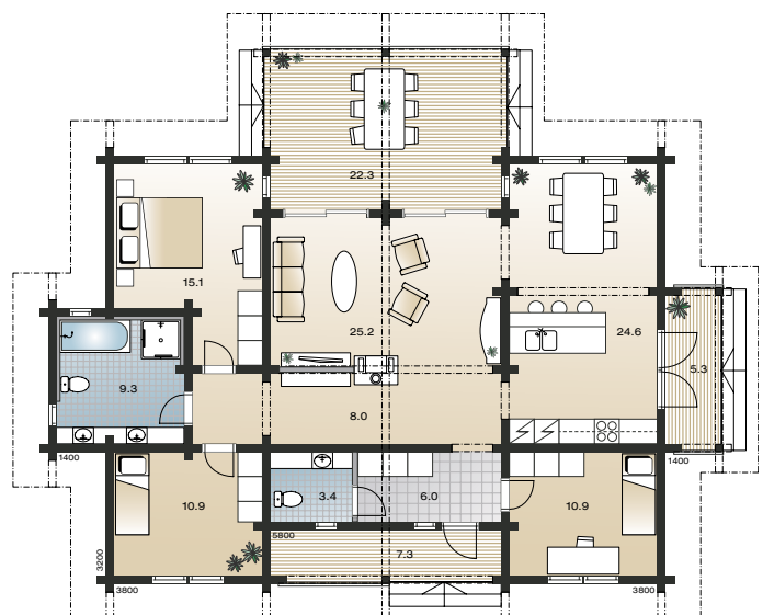
GROUND FLOOR 1:200
