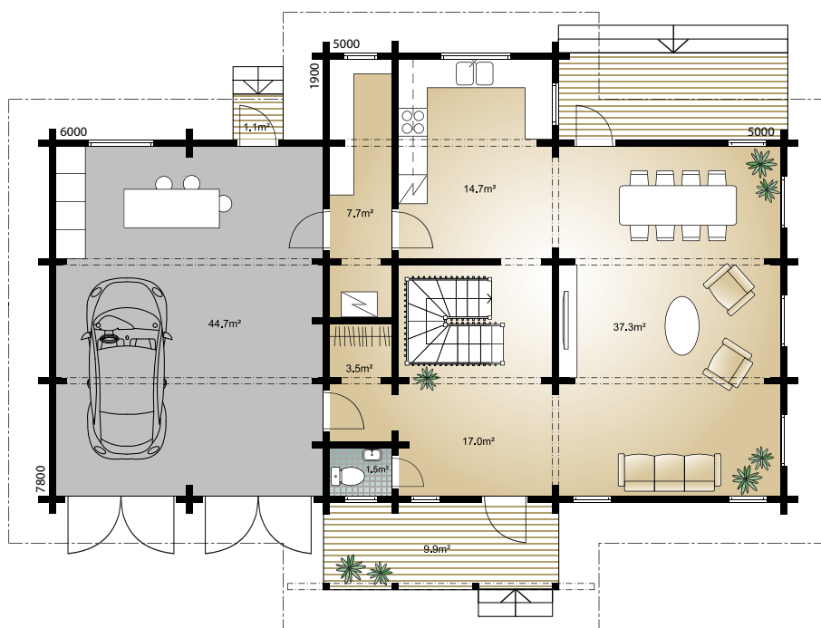
GROUND FLOOR 1:150
