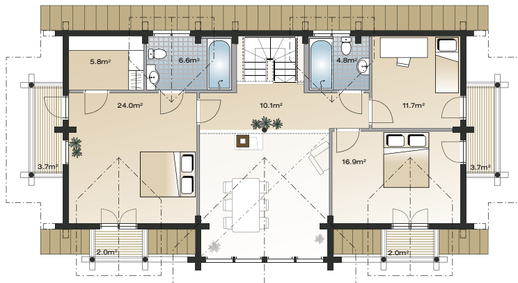
FIRST FLOOR 1:200
