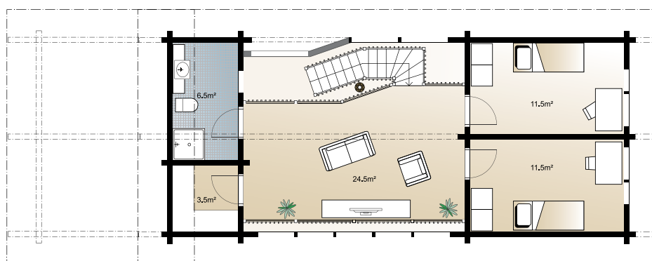
FIRST FLOOR 1:150
