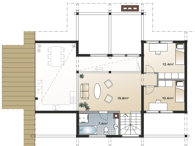
FIRST FLOOR 1:200
