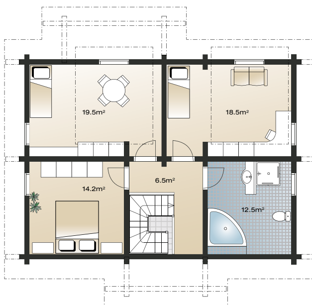
FIRST FLOOR 1:150
